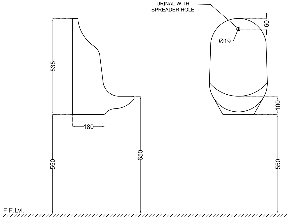
SIDE VIEW
