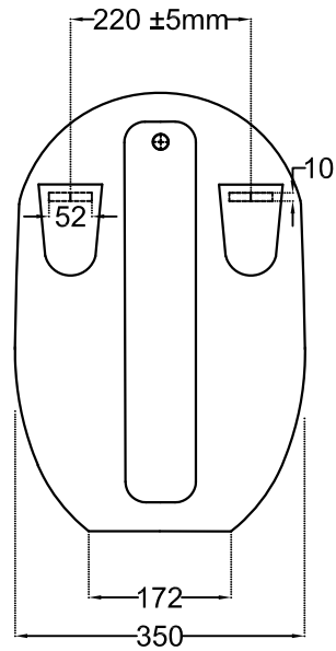
BACK VIEW
