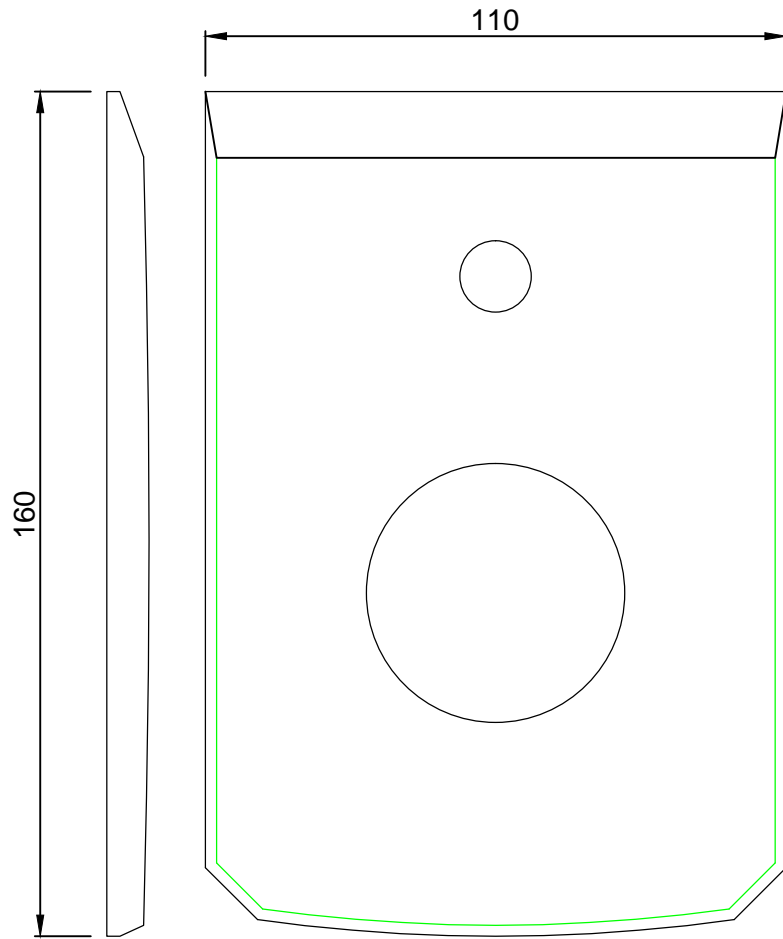
WALL FLANGE
