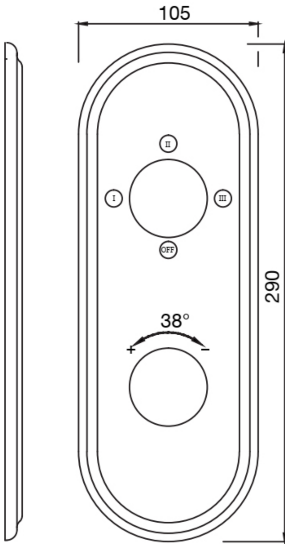
WALL FLANGE
