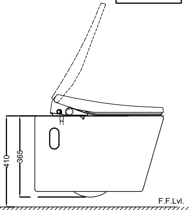
SIDE VIEW
