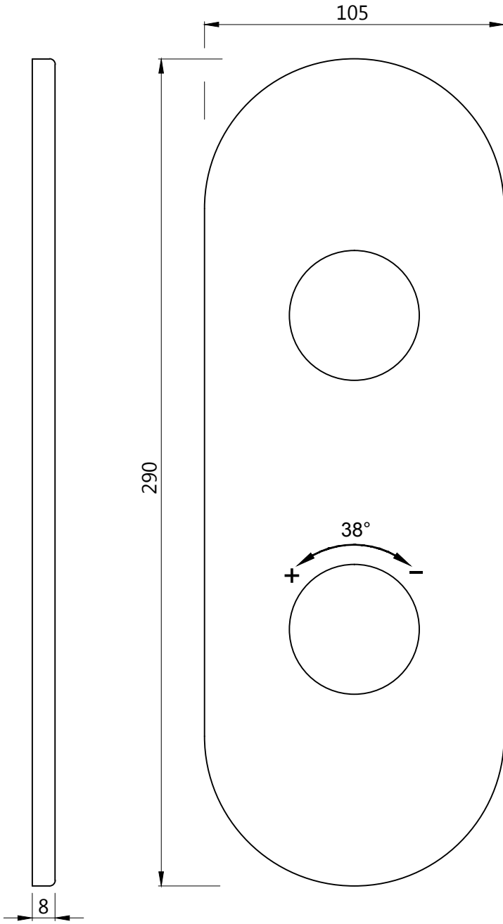
WALL FLANGE
