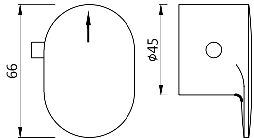
THERMOSTATE HANDLE
