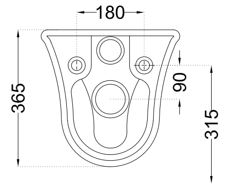
BACK VIEW
