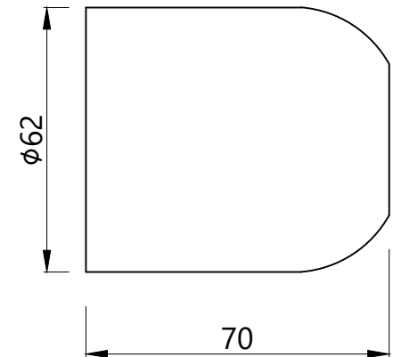
SLEEVE
