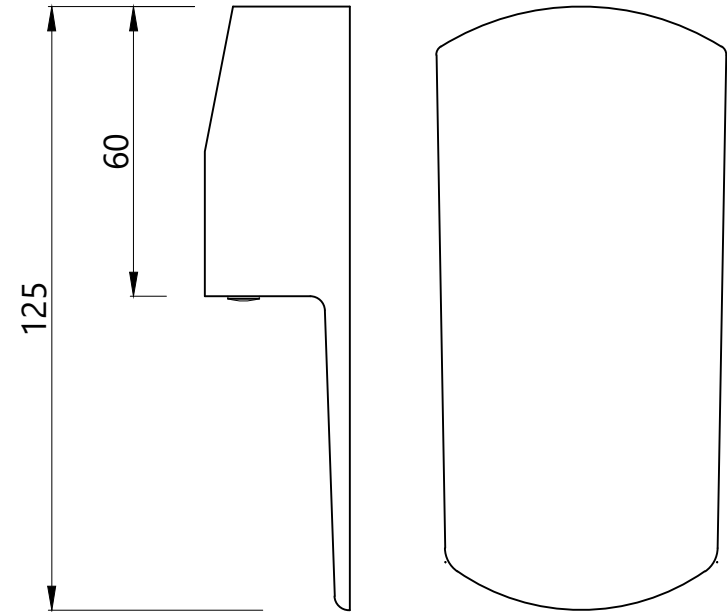
OPERATING LEVER
