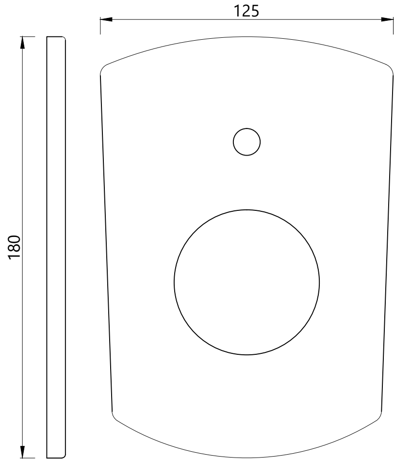
WALL FLANGE
