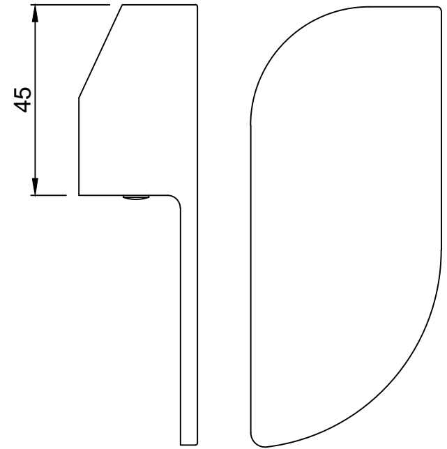
OPERATING LEVER
