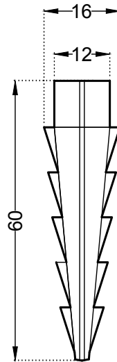
PVC SLEEVE
