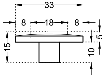
PVC WASHER VIEW
