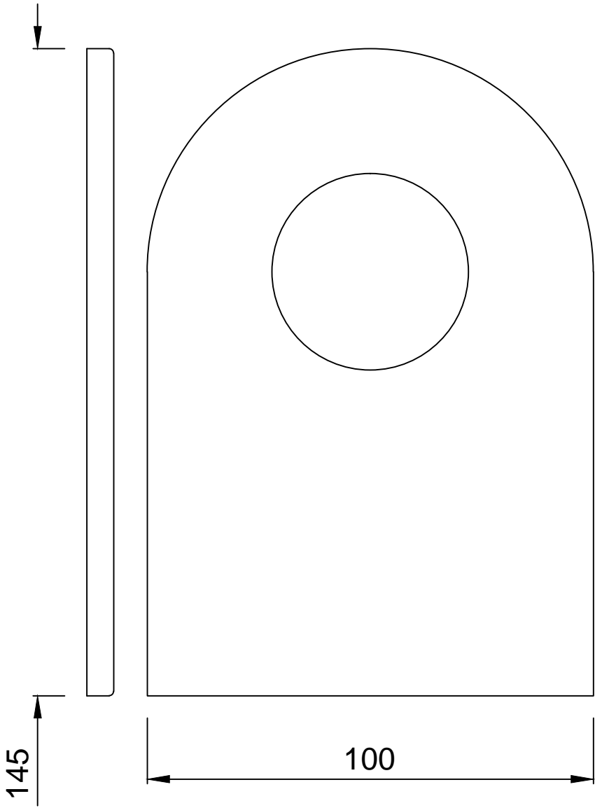
WALL FLANGE
