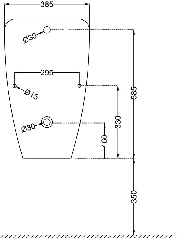
BACK VIEW
