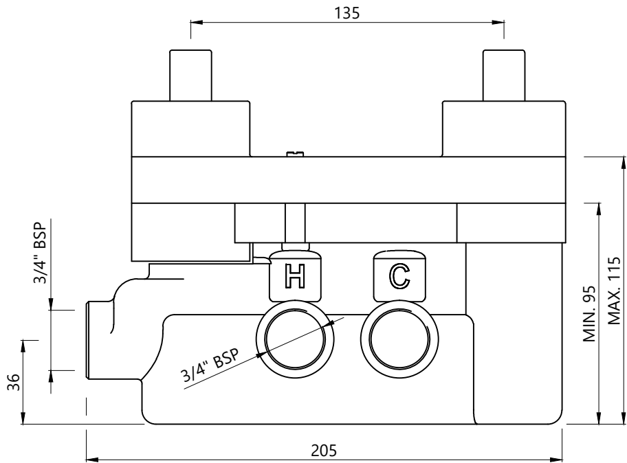
THERMOSTATIC SHOWER MIXER BODY
