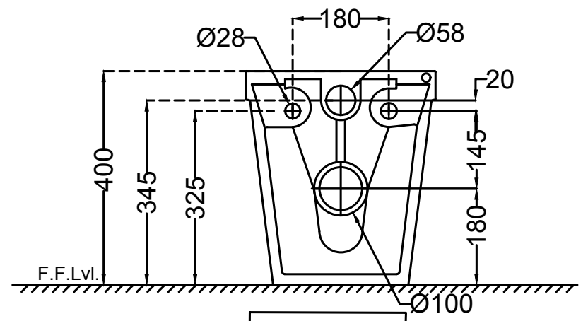
BACK VIEW
