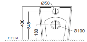
BACK VIEW
