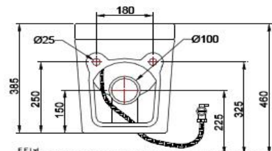
BACK VIEW
